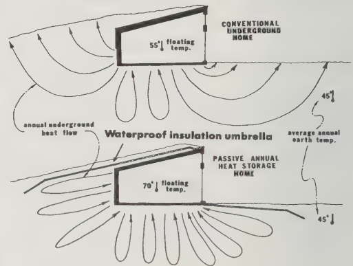
PASSIVE ANNUAL HEAT STORAGE
